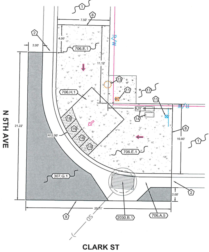
PROPOSED PLAN
