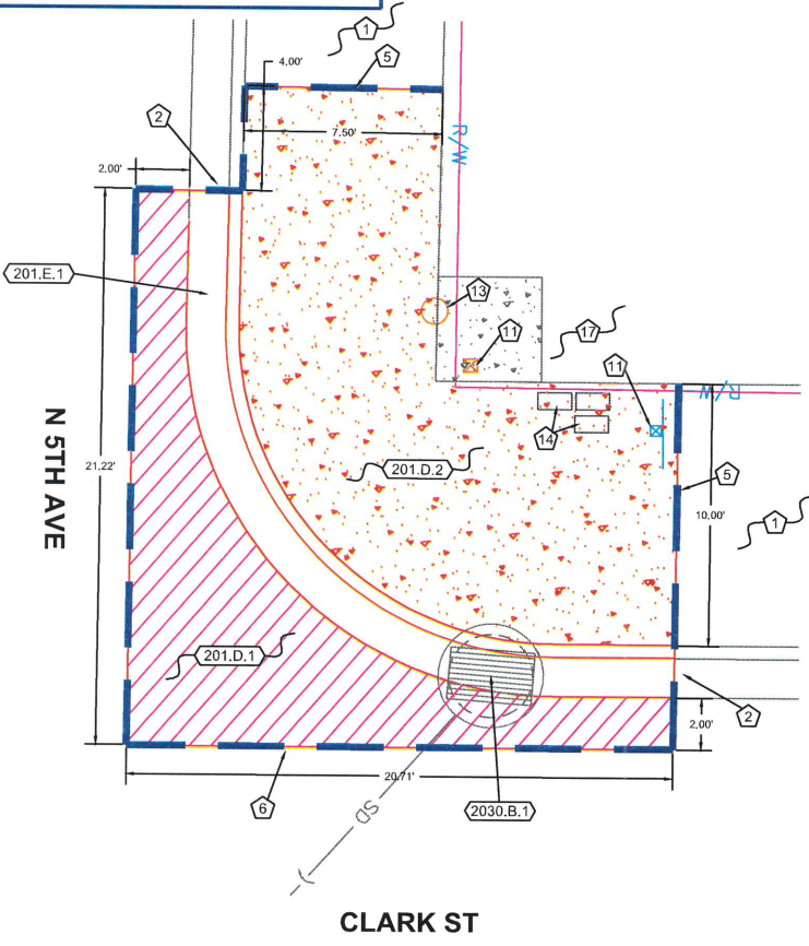
DEMOLITION PLAN
