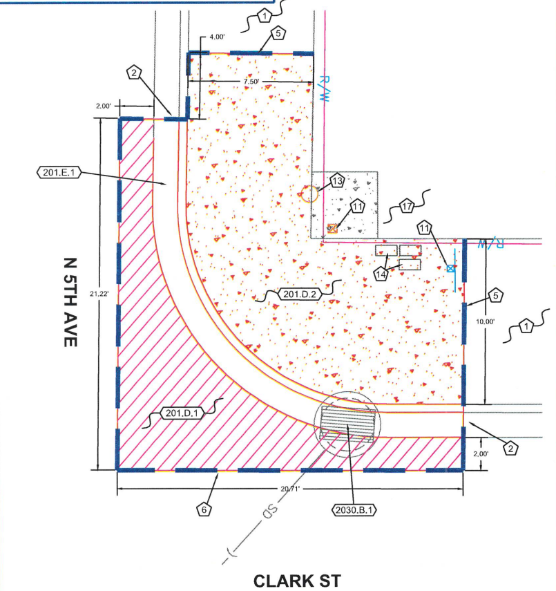
DEMOLITION PLAN
