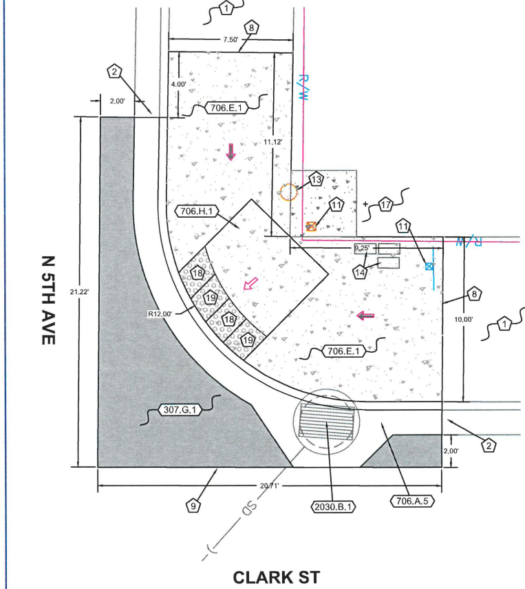
PROPOSED PLAN
